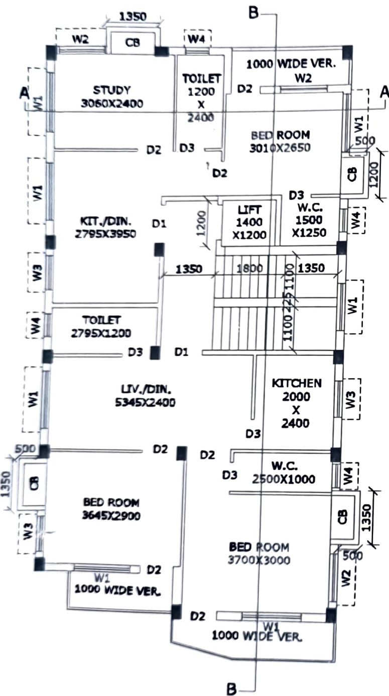
1ST & 3RD FLOOR PLAN
